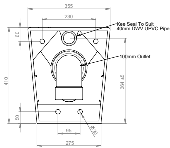
MODEL PCS Side and Rear Elevation
