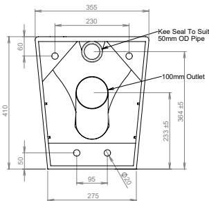
MODEL PCP Side and Rear Elevation
